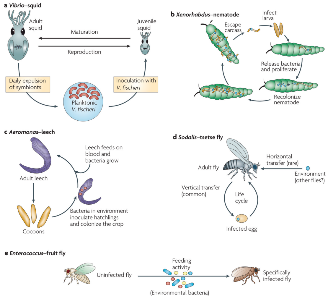
Figure 3. Simplified life cycles of five symbioses
