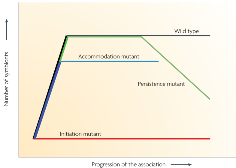
Figure 4. categories of colonization mutants
